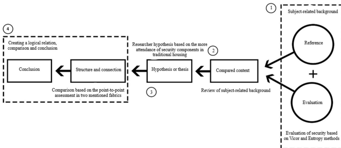
Fig. 1. Theoretical Framework
